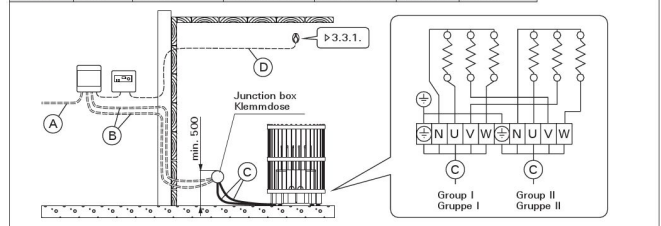
Electrical connections
